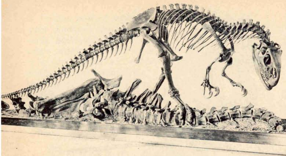
MEAT-EATING DINOSAUR — Photo shows the dinosaur, Allosaurus fragilis , mounted as if feeding upon a brontosaurus skeleton. This allosaurus skeleton from the Morrison beds of Colorado is about thirty feet long.
