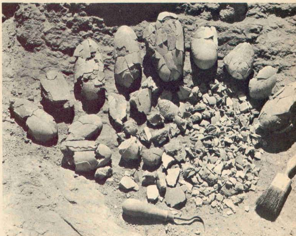
ANCIENT EGGS — These eggs of the dinosaur, Protoceratops , were discovered in Outer Mongolia. Paleontologists puzzle about how they were preserved.
