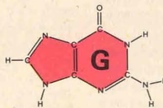
GUANINE
