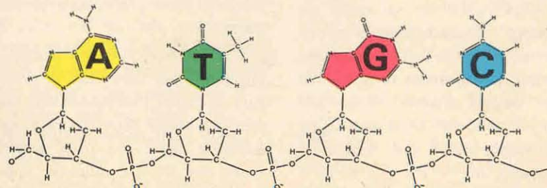
THYMINE
